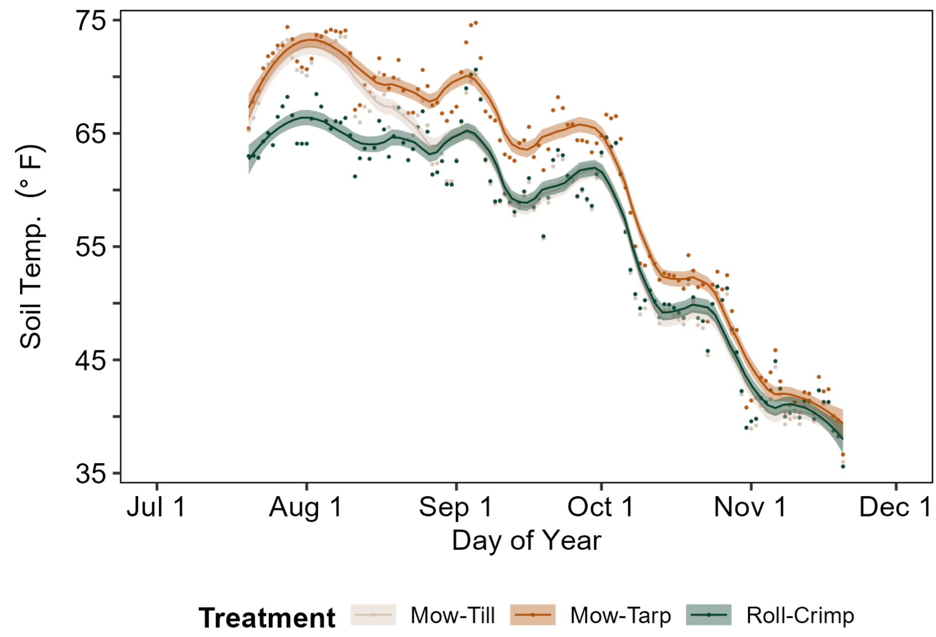
Figure 3. Mean daily soil temperature ( ^{\circ}F ) observations for each treatment throughout the study period.
